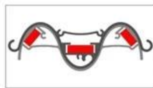
3 PTC HEATERS
